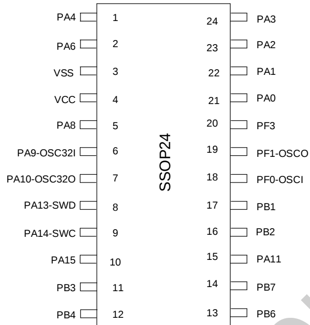
Figure 3-5 SSOP24 Pinout3 PY32F032E3xM7 (Top view)
